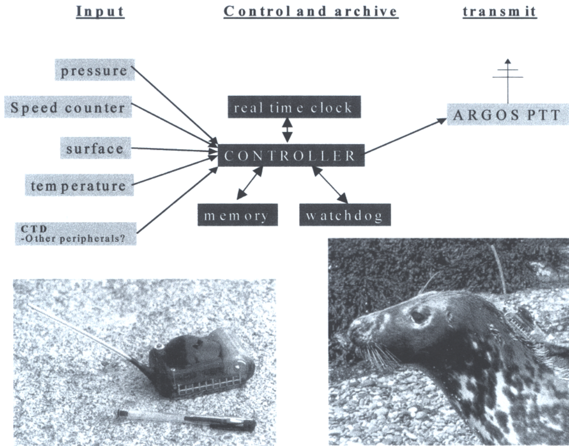
FIG. 1. A schematic of the functional elements within the Sea Mammal Research Unit's satellite relayed data logger along with photos of one version of the tag. The device contains a controller programmed in a high level language that controls data collection and storage functions as well as data compression and transmission strategies. It sends messages via the transmitter to the Argos system which relays information to ground stations for automatic dissemination to a local database. The left hand photo shows the tag in the form typically used on seals. The right-hand photo shows the tag glued to the fur of a yearling gray seal ( Halichoerus grypus ).
